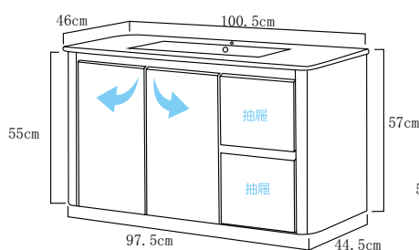
E8310/E8310-1 不鏽鋼櫃組 1005x460x570mm $60,000 E8312/E8312-1 不鏽鋼櫃組 1205x460x570mm $70,000
